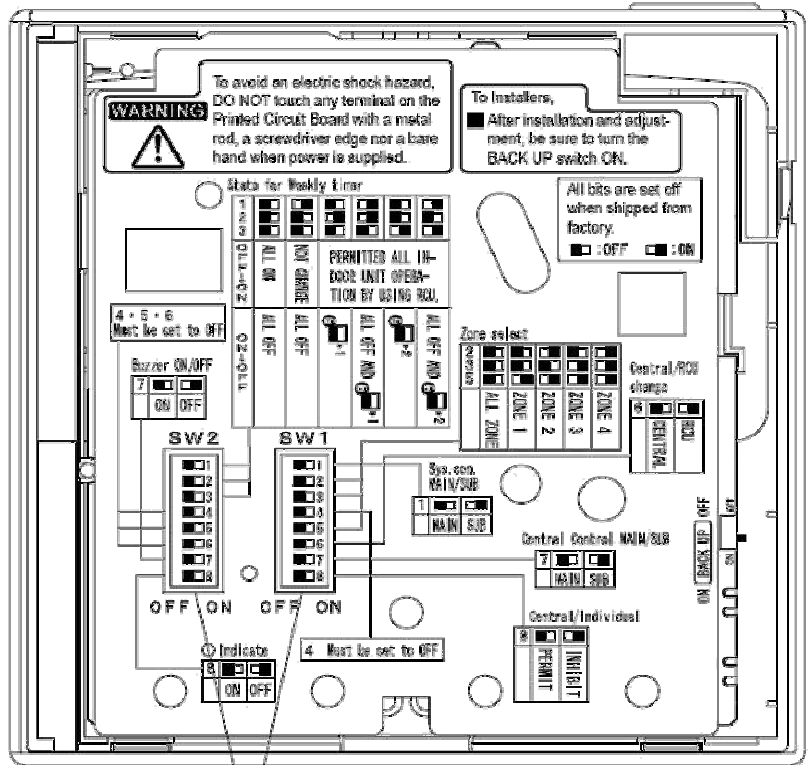
PCB of the control unit
